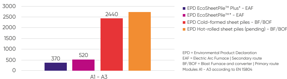
Global Warming Potential [kg CO 2 e / metric ton of sheet pile]
