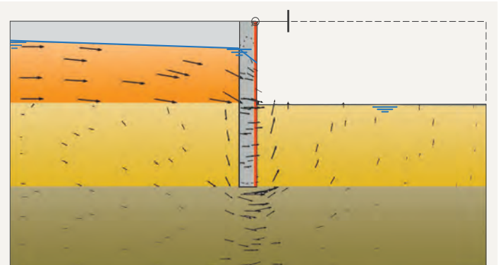
Ultimate flow field with phreatic line Extreme velocity 4.21E-05 units Case 2
